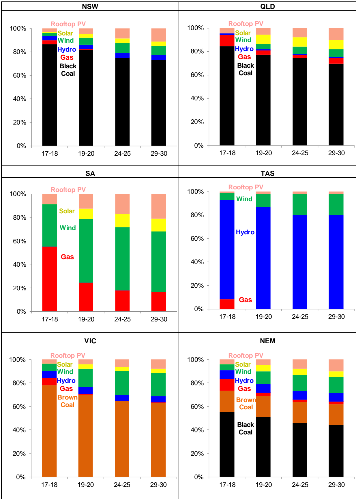
Chart 15: Panel of projected jurisdictional energy mix (sent out) – Guarantee scenario
